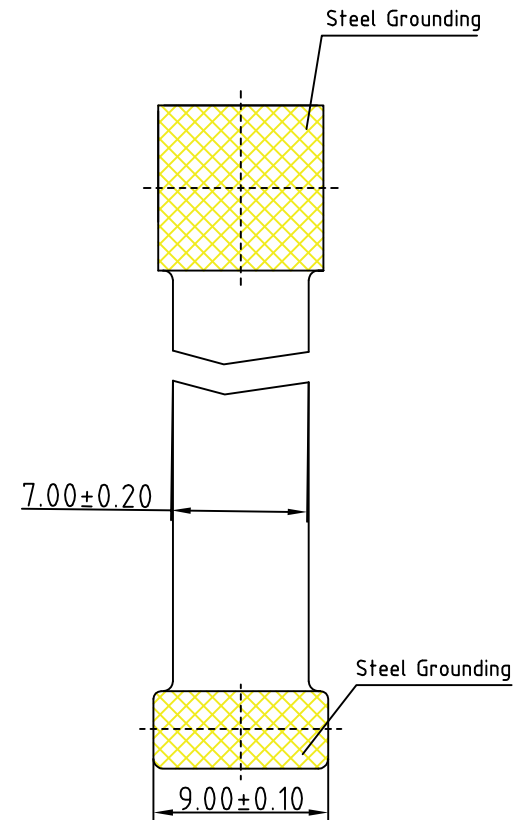
BOTTEM VIEW
